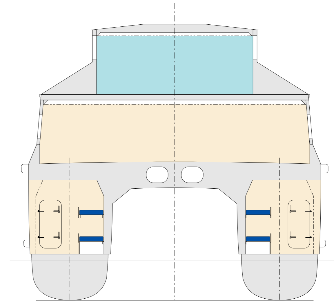
TYPICAL SECTION
