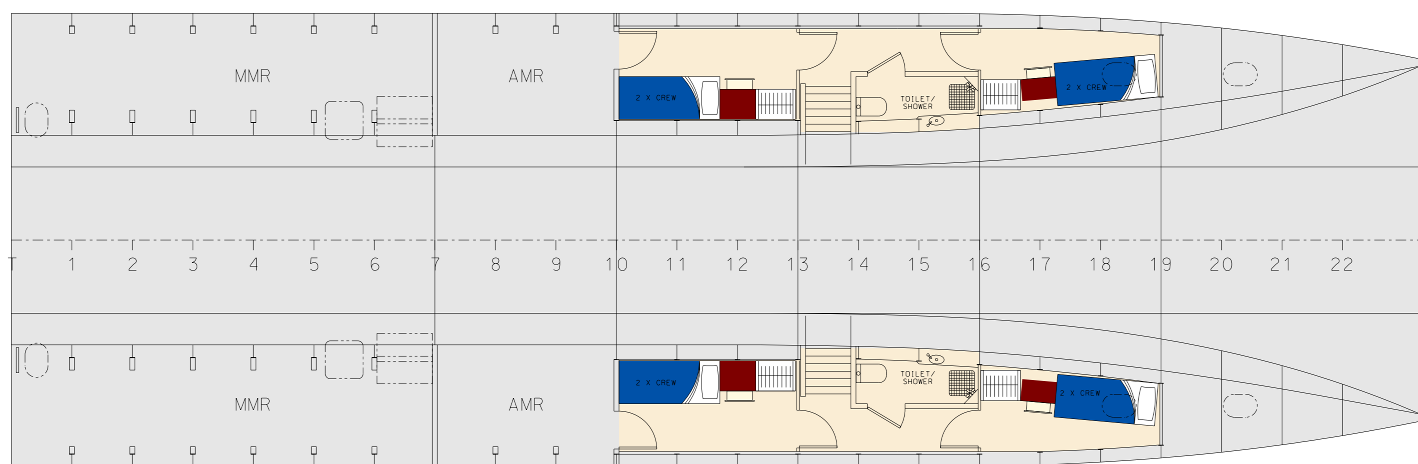
PLAN BELOW DECKS
