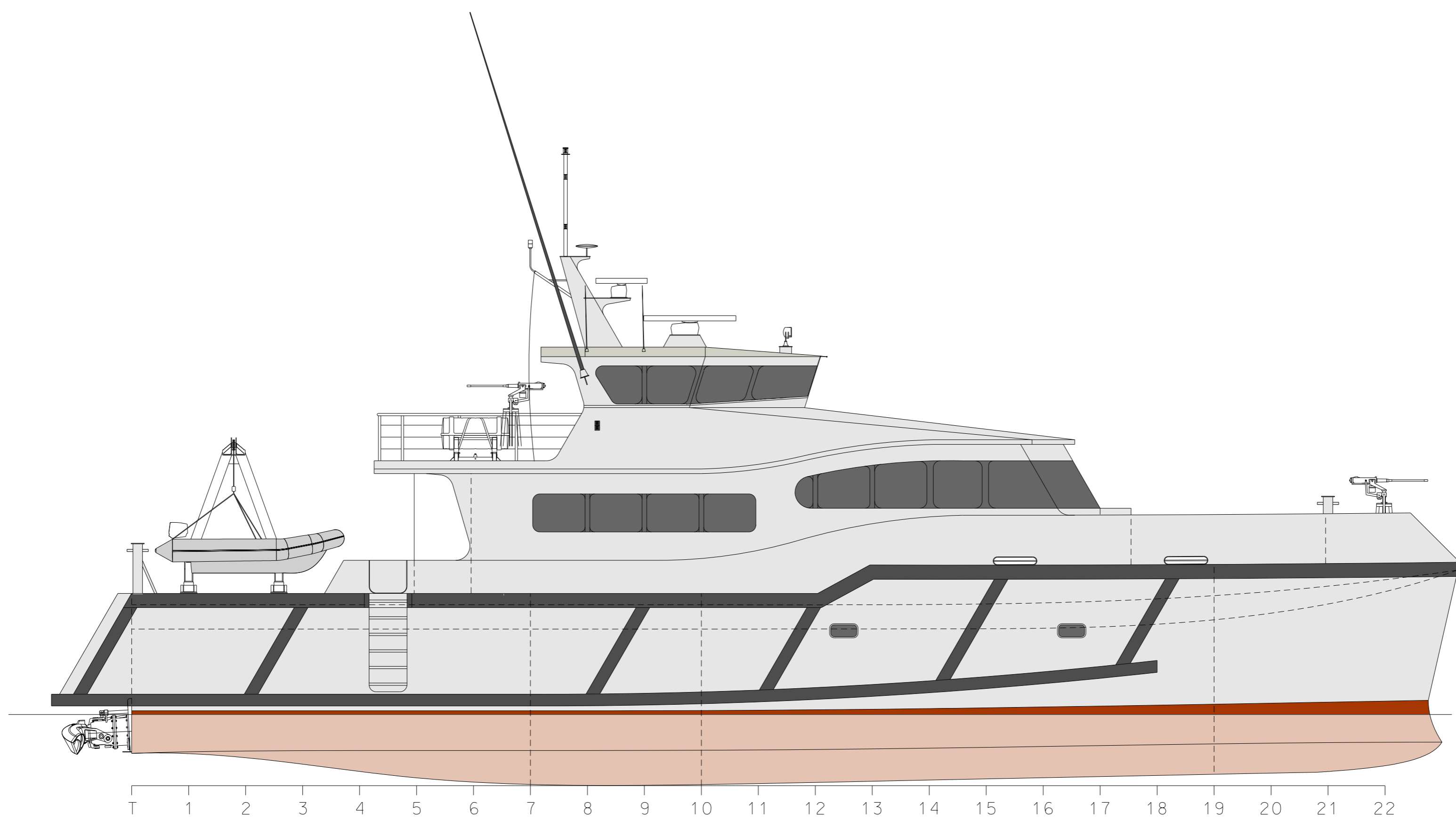
OUTBOARD PROFILE
