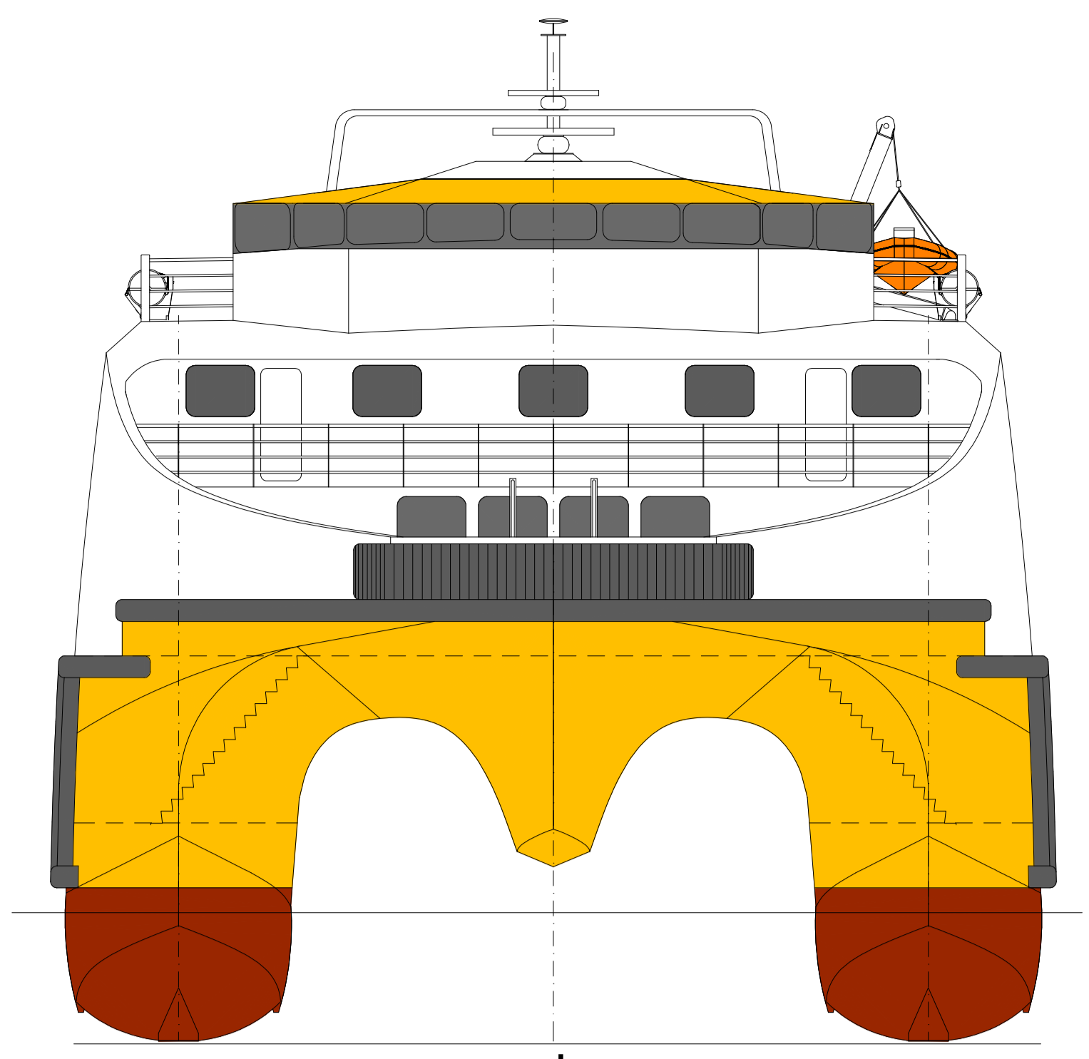
FWD ELEVATION
