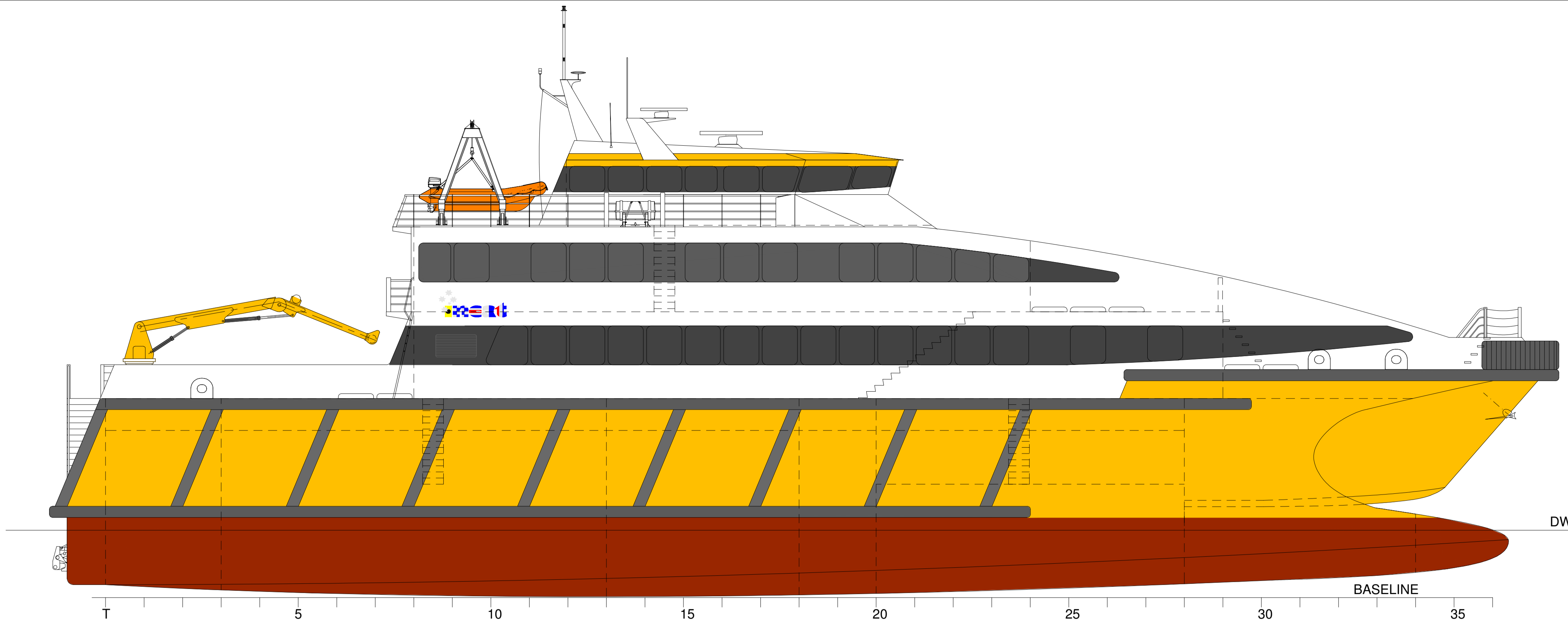
OUTBOARD PROFILE
