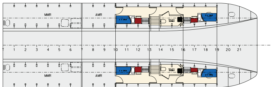
PLAN BELOW DECKS
