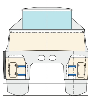
MIDSHIP SECTION
