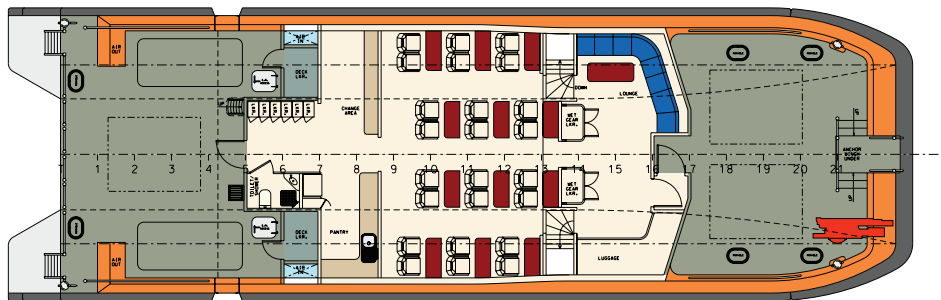
MAIN DECK PLAN
