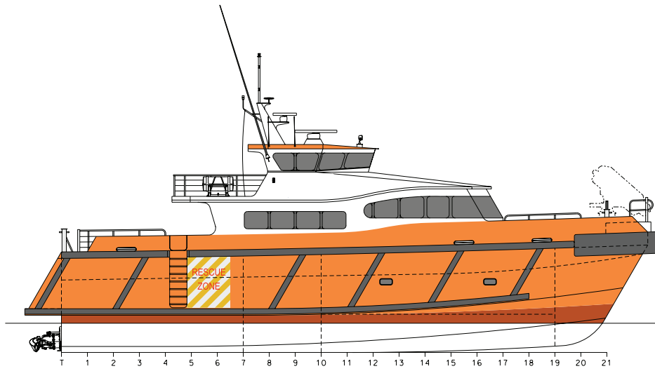
OUTBOARD PROFILE
