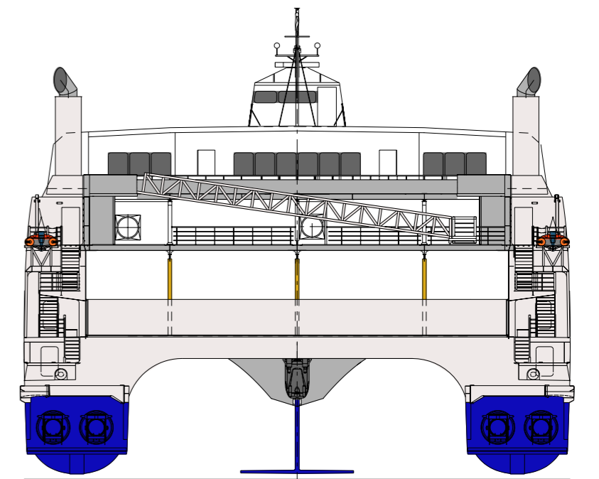
VIEW FROM ASTERN
