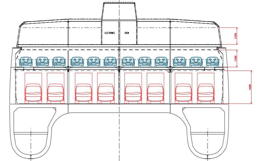
MIDSHIP SECTION
