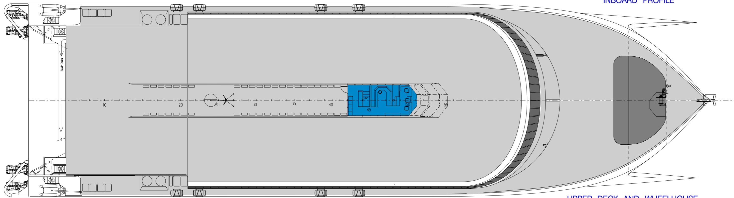
UPPER DECK AND WHEELHOUSE
