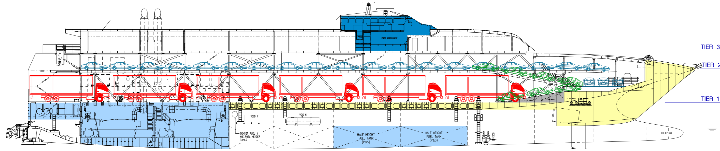
INBOARD PROFILE
