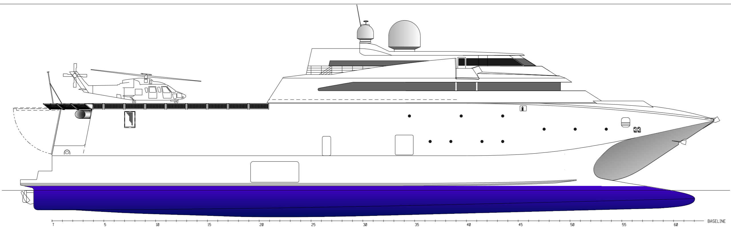
OUTBOARD PROFILE
