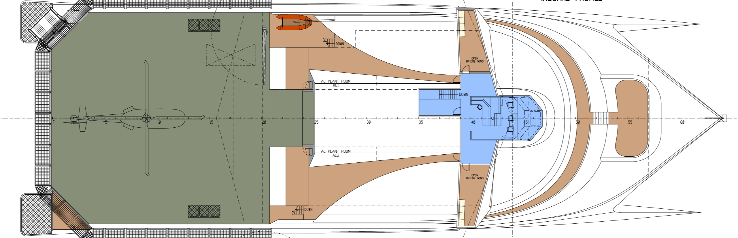
WHEELHOUSE AND UPPER DECK PLAN
